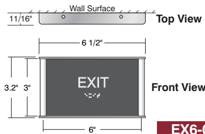
6" x 3" Egress Identification Tactile Copy with Braille
