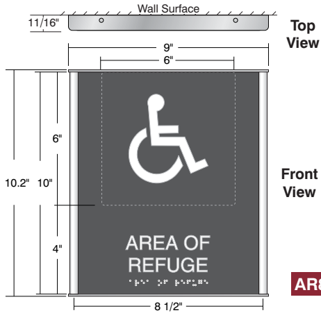
8 1/2" x 10" Area of Refuge Tactile Pictogram and Copy with Braille
