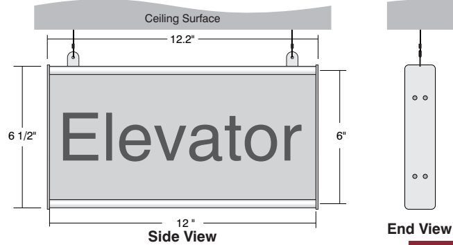
6" x 12" Suspended Ceiling Mount No Tactile Copy or ADAAG Braille Requirements Single or Double Faced
