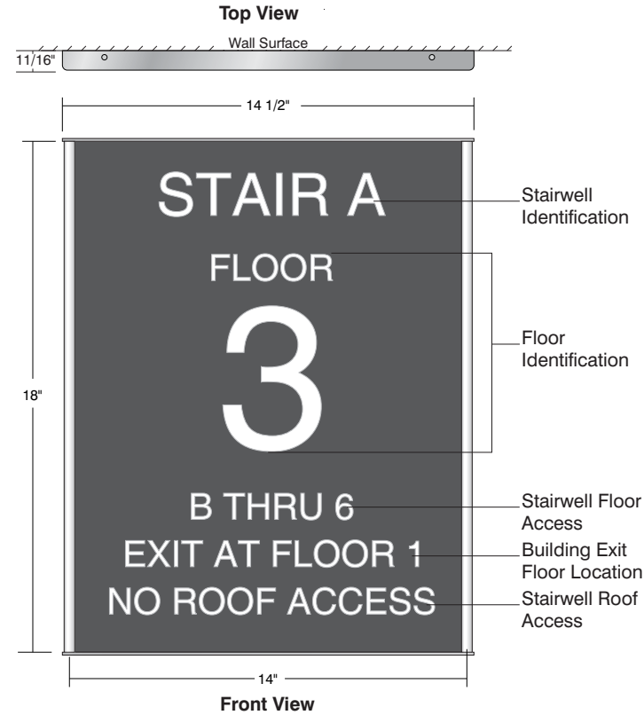
14" x 18" Interior Stairwell Sign Tactile Copy - No ADAAG Braille Requirements ADAAG Required in Buildings 4 stories and Higher
