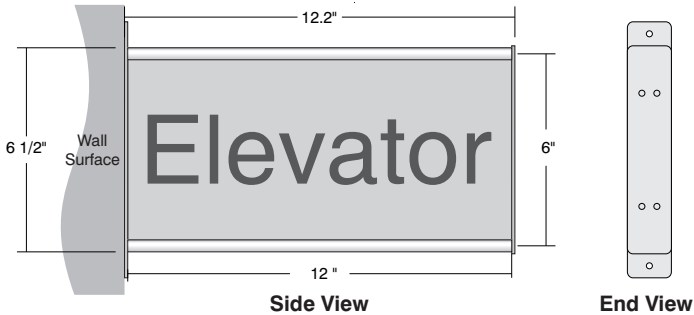
6" x 12" Projection Wall Mount No Tactile Copy or ADAAG Braille Requirements Single or Double Faced
